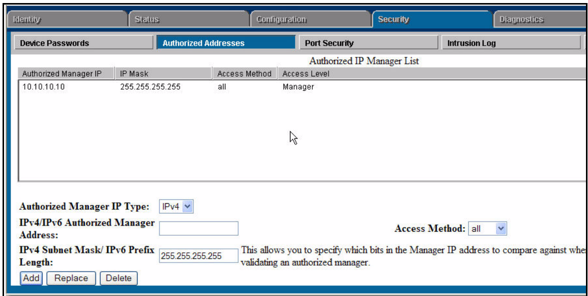
Figure 14-5. Example of Configuring Authorized Manager Access Method in the Web Interface
